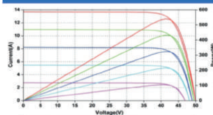
Current-Voltage and Power-Voltage Curves at Different Irradiances
